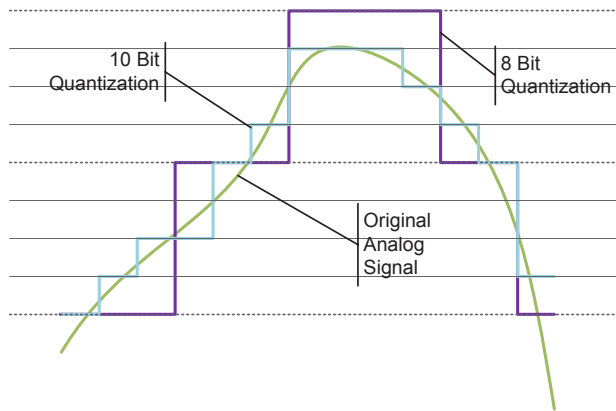
Figure 1 – 10-bit vs. 8-bit quantization.
