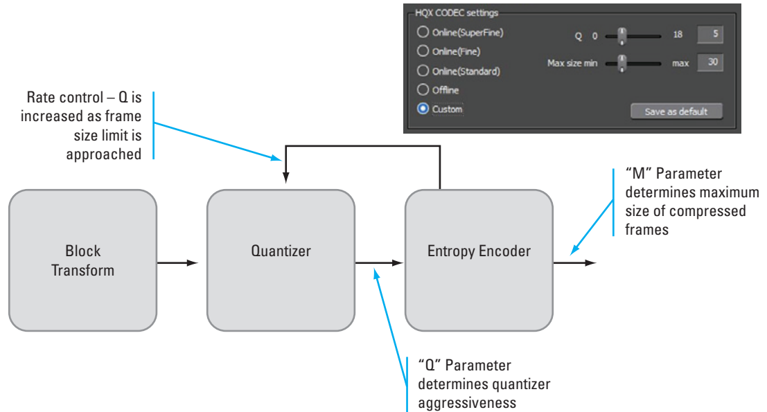
Figure 5 – HQX codec architecture.
