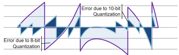
Figure 2 – Comparison of quantization errors.
